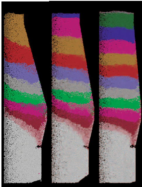
(a) Shaft angle: 75° (b) Shaft angle: 80° (c) Shaft angle: 85° 図6 シャフト角が固体流れに及ぼす影響の計算結果 Fig.6 Calculated effects of shaft angle on solid flow
